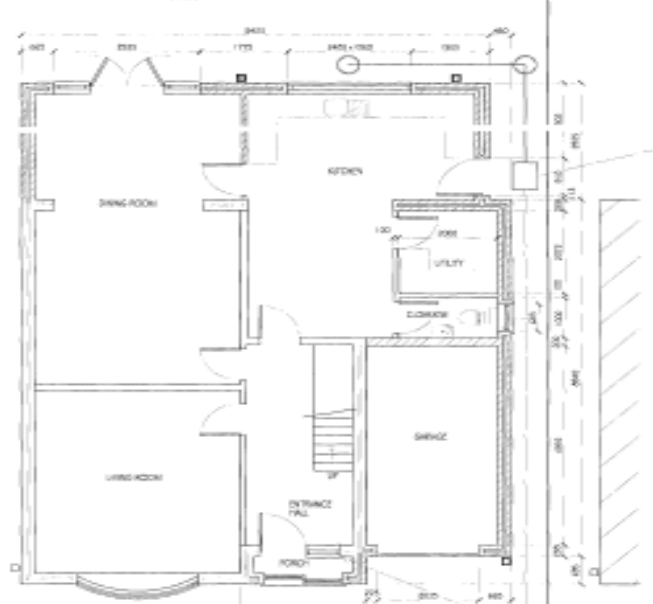
GROUND FLOOR PLAN - PROPOSED 1:80
