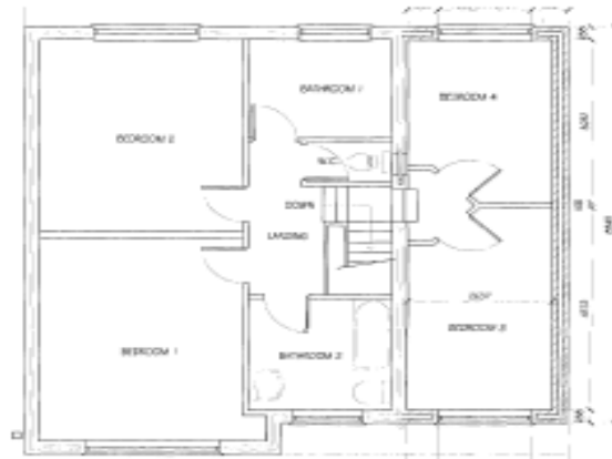
FIRST FLOOR PLAN - PROPOSED 1:80
